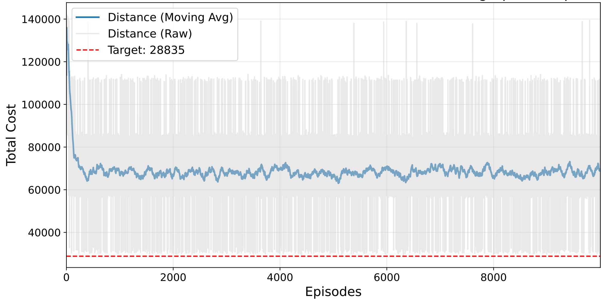
Final GAUSSIAN PROCESS Masked AutoRL-SOP Training - p43.3.sop
